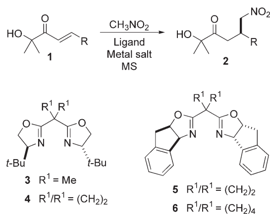
Scheme 1. Conjugate addition of nitromethane to \alpha' -hydroxy enones 1 under Lewis acid catalysis.
