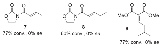
Figure 1. \alpha,\beta -Unsaturated carboxylic acid surrogates examined for the base-free reaction with nitromethane. Conditions: ligand 5 :Mg(OTf) 2 (10 mol %), 4 Å MS, room temperature, 4–5 days.
