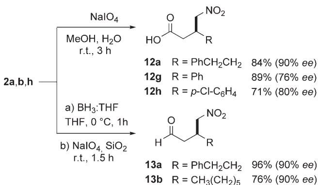
Scheme 3. Elaboration of adducts into \gamma -nitro carboxylic acids and aldehydes.
