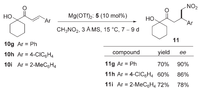
Scheme 2. Improved results with structurally modified \alpha' -hydroxy enone 10 .
